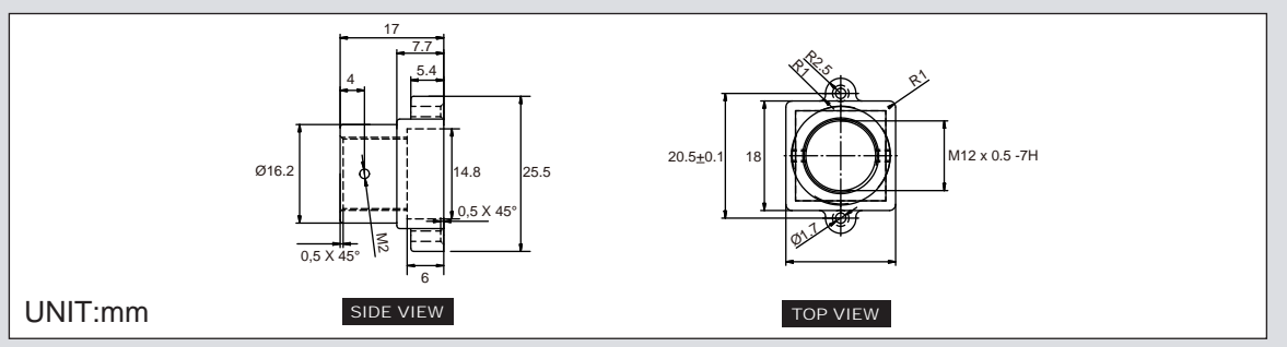
MS-9431M-01 METAL BOARD LENS HOLDER
