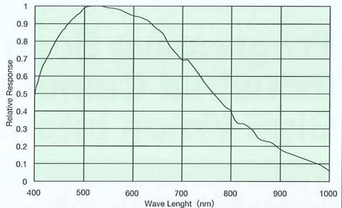
Spectrum sensitivity characteristic (Example of representative characteristic)
